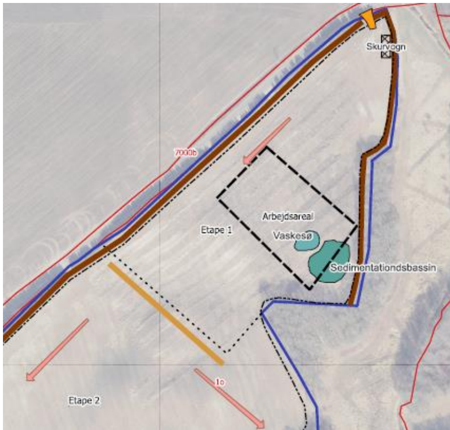
Figur 1: Situationsplan
